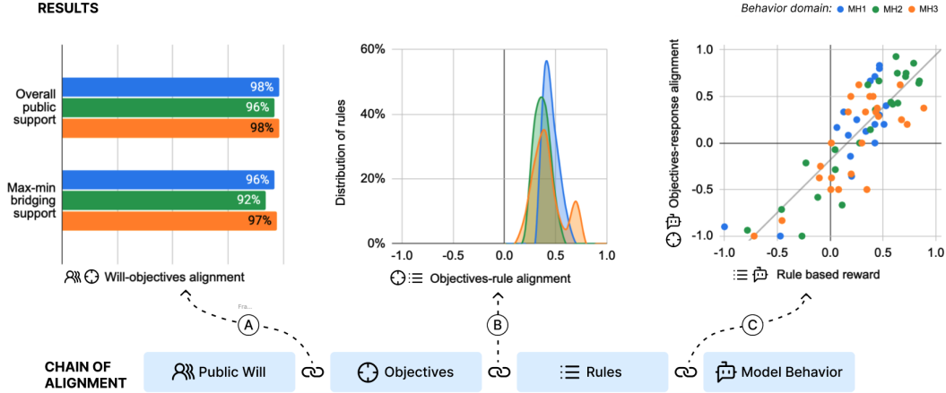
Figure 1: Our approach produces objectives and rules that form a “chain of alignment” linking model behavior to public will (bottom). We test our approach across three domains of LM behavior, and evaluate each link in the resulting alignment chain (top): A) Public support for the objectives gives a measure of their alignment with public will . B) The distribution of rules ’ alignment with the objectives is produced by domain experts assessing each rule’s likelihood to help achieve the objectives. C) The rules ’ ability to measure if model behavior aligns with the objectives is assessed by comparing the output of an LM-graded rule based reward (x-axis) with domain expert assessments of alignment with objectives (y-axis) for a diverse sample of {user prompt, LM response} pairs.
